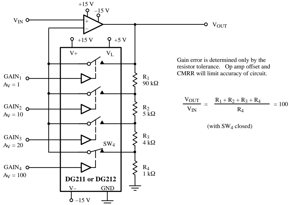
Figure 6. Precision-Weighted Resistor Programmable-Gain Amplifier
